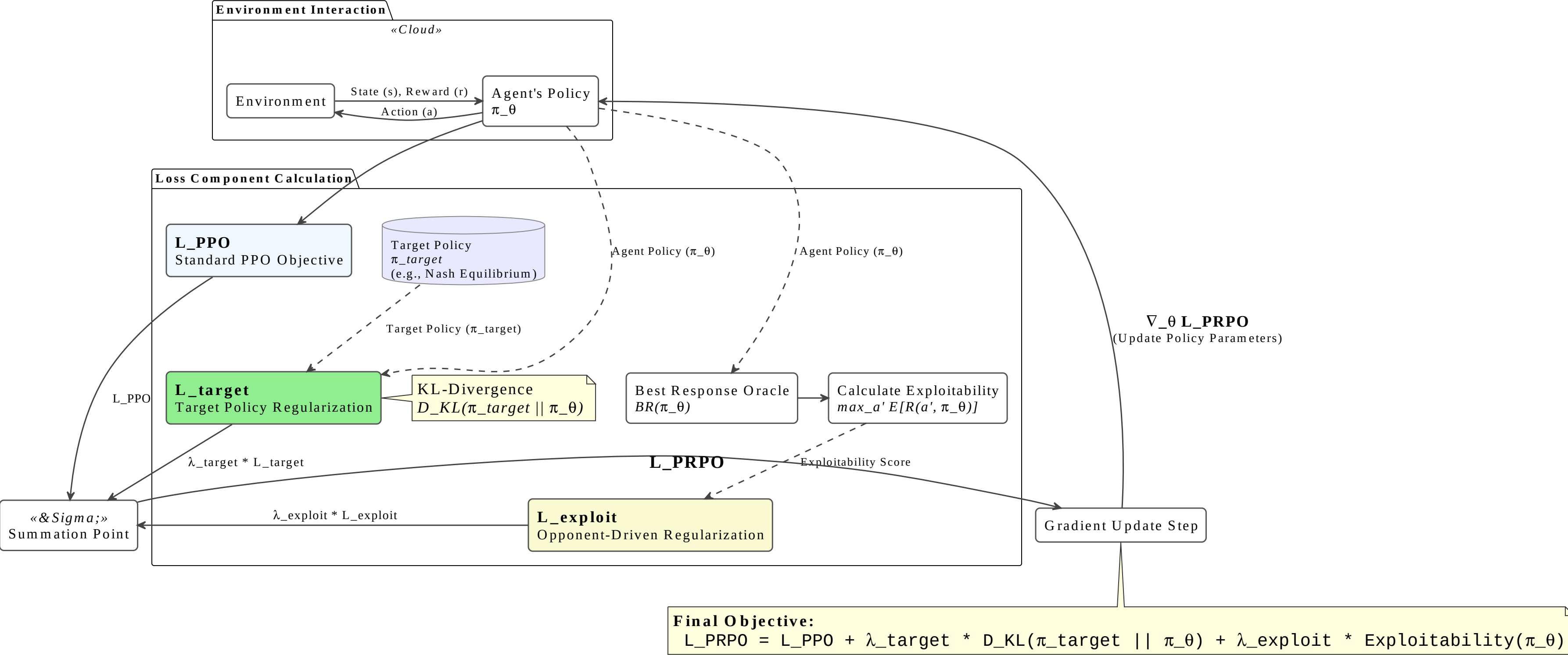
Figure 2: Conceptual Diagram of the Unified PRPO Objective
